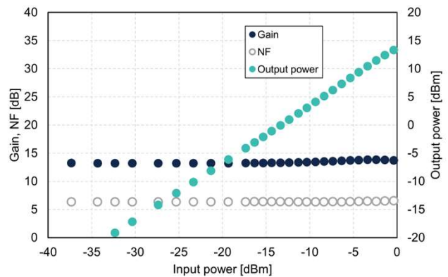
Gain/NF/output power vs. input power @1480nm
