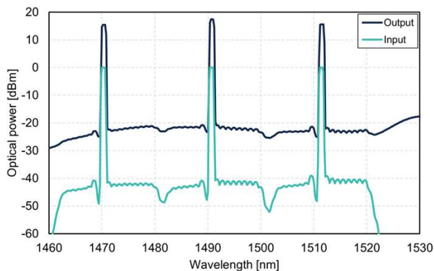
Input power/Output power vs. wavelength
